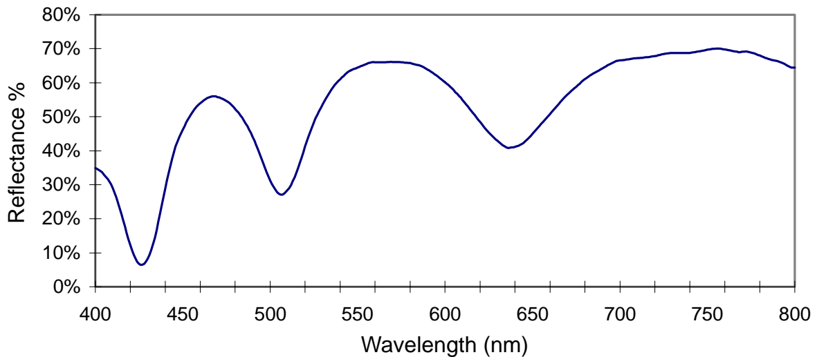
Figure 9: Measured reflectance of a FPMI using 300 nm-SiN/40 nm-Ag mirrors with an air gap of about 1 \mu\text{m} (without adjustment of parallelism).
