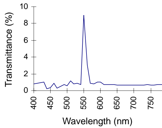
Figure 7: Optical transmittance measured for an air cavity gap of about 500 nm and silver mirrors with thickness of 40 nm.
