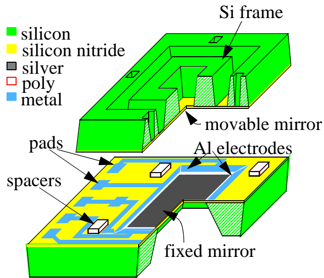
Figure 1a: Fabry-Perot MicroInterferometer (FPMI).
