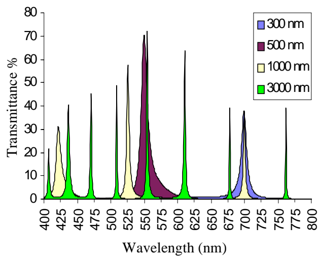
Figure 3: Simulated transmittance for different cavity gap widths.
