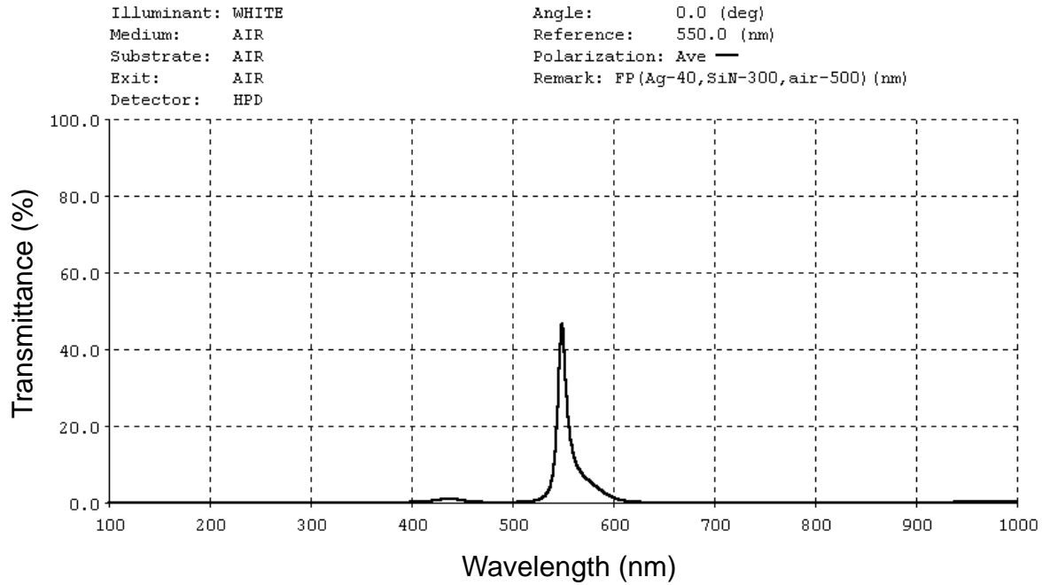
Figure 8: Simulated transmittance of a FPMI using 300 nm-SiN/40 nm-Ag mirrors with an air gap of 500 nm.
