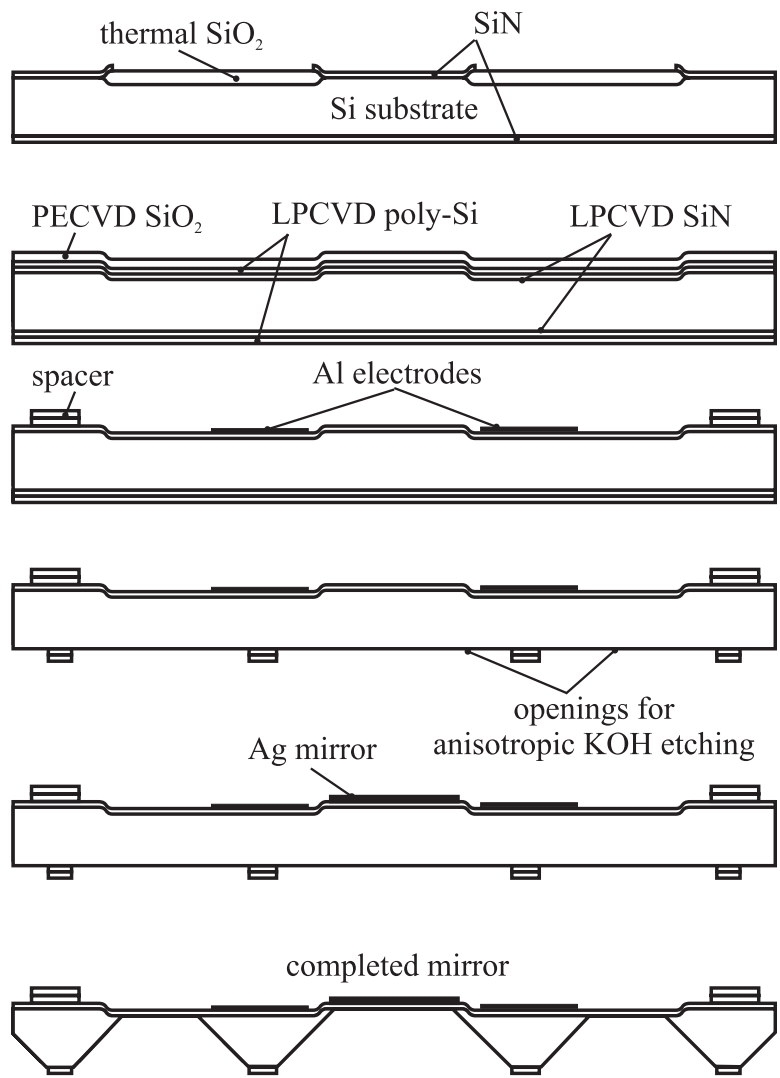
Figure 5: Schematic fabrication sequence.
