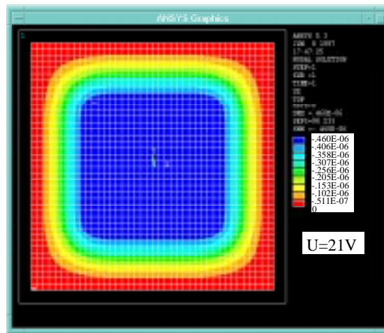
Figure. 2: FEM simulation of the SiN-membrane/Si frame deflection.
