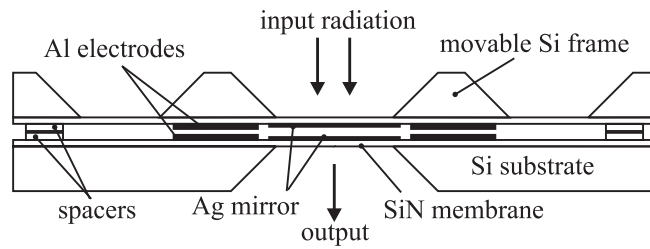
Figure 1b: Cross-section of the micromachined F-P optical filter.
