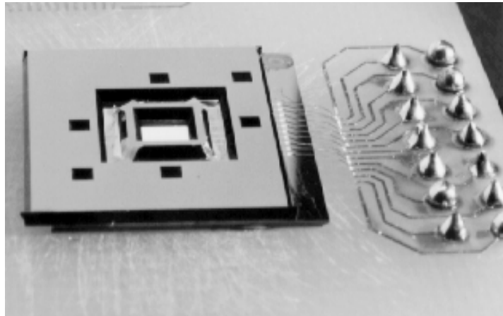
Figure 6: Photograph of the fabricated FPMI.
