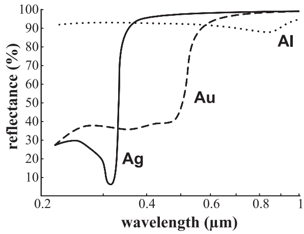
Figure 4: Optical reflectance of Ag, Al and Au.
