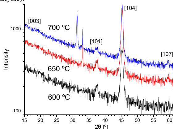
Fig 3: XRD spectrogram of three \text{LiCoO}_2 films annealed at different temperatures (600 °C, 650 °C and 700 °C).
