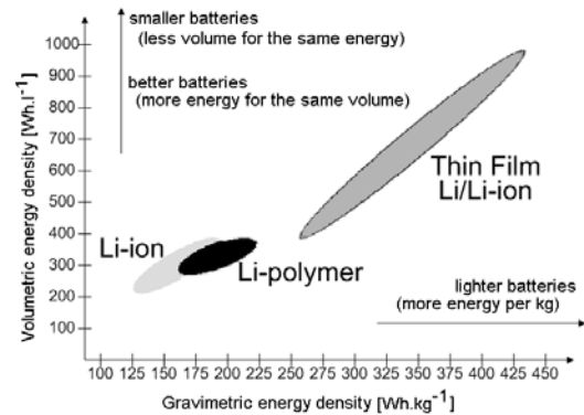
Fig 1: Size and capacity with different battery technologies.
