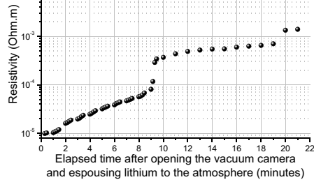
Fig 7: Evolution of lithium resistivity in contact with air.
