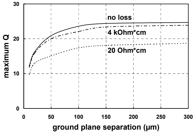
Figure 11: Quality factor of a 17-nH spiral inductor (in 4- \mu\text{m} Al metallisation) vs. the separation of a metal ground plane for three different substrate resistivities.
