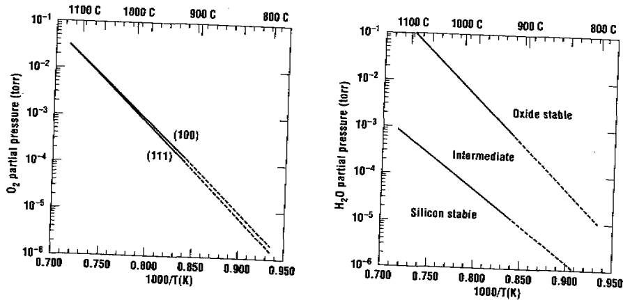
Figure 14.2 Stability diagram for the surface of silicon and silicon dioxide as functions of the temperature and the partial pressure of oxygen and water vapor. The curve for water vapor has an intermediate region where both surfaces can coexist (redrawn using data from Ghidini and Smith, and Smith and Ghidini).
