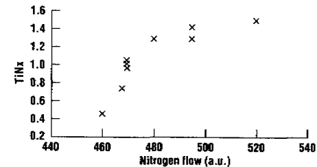
Figure 12.27 Resistivity and composition of reactively sputtered TiN as a function of the N 2 flow in the sputtering chamber (after Tsai, Fair, and Hodul, reprinted by permission, The Electrochemical Society, and Molarius and Orpana, reprinted by permission, Kluwer Academic Publishing).
