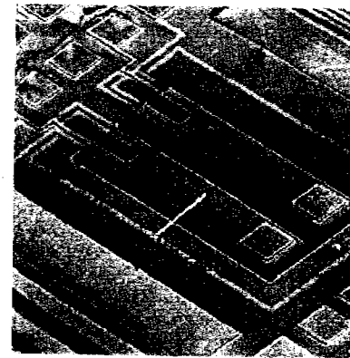
Figure 19.21 A pair of silicon cantilever beams used to detect airborne contaminants prior to deposition of the polymer layer (after Baltes [47], © 1998 IEEE).
