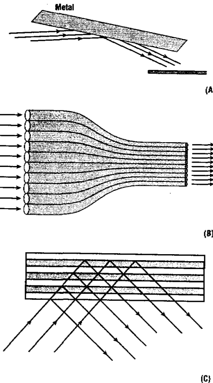
Figure 9.20 Possible choices for x-ray optics systems include glancing angle metal mirrors (A), Kumakhov lenses (B), and multilayer mirror (C).
