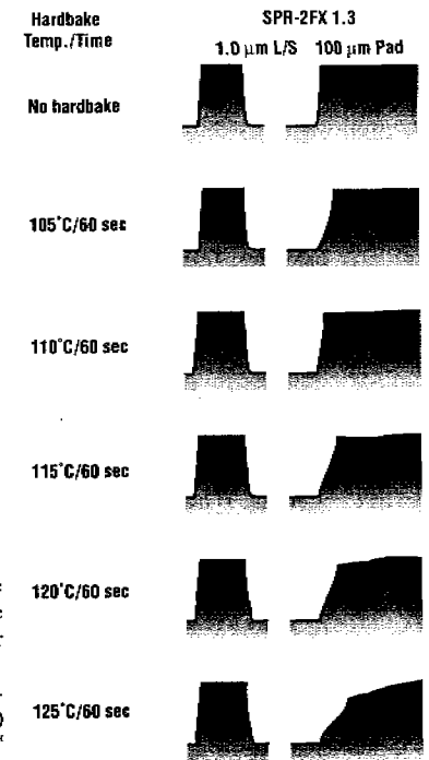
Figure 8.11 Resist profiles of a 1- \mu\text{m} line and space and a large feature in SPR-2FX resist for different hardbake temperatures (courtesy Shipley).
