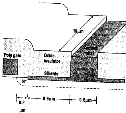
Figure 16.16 Cross section and dimensions of MOSFET example.
