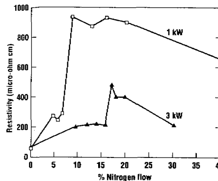
Figure 12.27 Resistivity and composition of reactively sputtered TiN as a function of the N 2 flow in the sputtering chamber (after Tsai, Fair, and Hodul, reprinted by permission, The Electrochemical Society, and Molarius and Orpana, reprinted by permission, Kluwer Academic Publishing).
