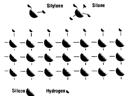
Figure 13.3 A simple model of the surface of the wafer during silane CVD includes adsorbed \text{SiH}_3 and \text{SiH}_2 .
