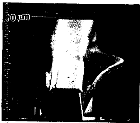
Figure 11.19 SEM micrographs of sidewall passivation films created in a \text{HClO}_2/\text{BCl}_3 plasma. In the upper micrograph, the photoresist and silicon posts have been removed by subsequent wet etching. The lower photo shows the sidewall film is partially peeled from the etched pattern (after Oehrlein et al., reprinted by permission, AIP).
