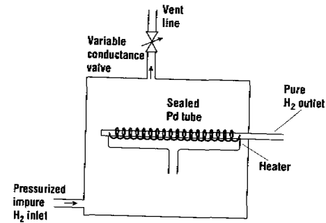
Figure 14.3 Schematic diagram of a palladium diffuser used for purifying hydrogen. Hydrogen diffuses through the high-temperature palladium barrier, while the impurities are swept out the vent line.
