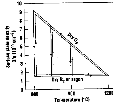
Figure 4.12 The Deal triangle showing the effects of a high-temperature inert (nitrogen or argon) postoxidation anneal on interface states and fixed charge density (after Deal et al. , reprinted by permission, The Electrochemical Society ).
