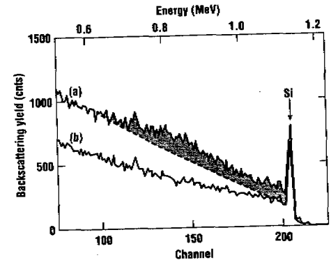
Figure 5.14 RBS spectra showing the backscattered He intensity as a function of energy. Curve (b) is an unimplanted wafer. The curve labeled (a) is a wafer after a 2 \times 10^{15} B implant at 200 keV. The dashed line represents the component of the spectrum corresponding to the remaining crystalline silicon. The shaded area represents the contribution of displaced atoms (reprinted by permission of Elsevier Science, after Schreutelkamp et al.).
