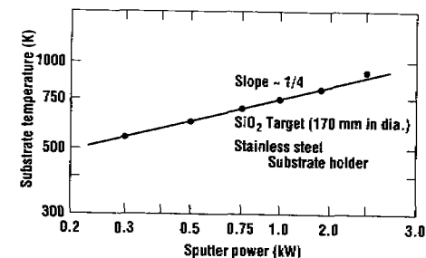
Figure 12.22 The temperature rise of substrates as a function of the plasma power for an argon RF plasma with an \text{SiO}_2 target (after Wasa and Hayakawa, reprinted by permission, Noyes Publications ).
