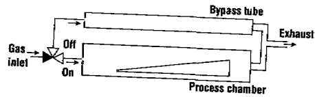
Figure 14.22 Run/vent gas switching used to avoid large gas transients.
