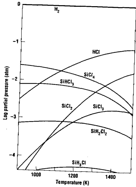
Figure 14.5 Equilibrium partial pressures in the Si-Cl-H system at 1 atm and a Cl to H ratio of 0.06 (after Bloem and Claasen, reprinted by permission, Philips).
