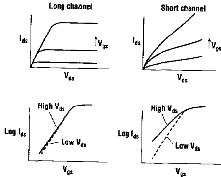
Figure 16.11 I - V characteristics of MOSFETs comparing long- and short-channel behavior. Typical threshold voltage dependence on gate length.
