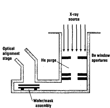
Figure 9.18 Simple proximity x-ray lithography aligner. The basic system is very similar to optical proximity systems.
