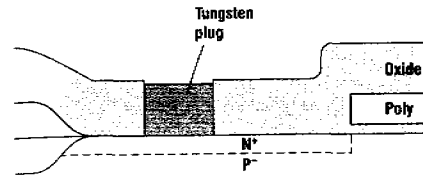
Figure 15.27 Tungsten plug structure.
