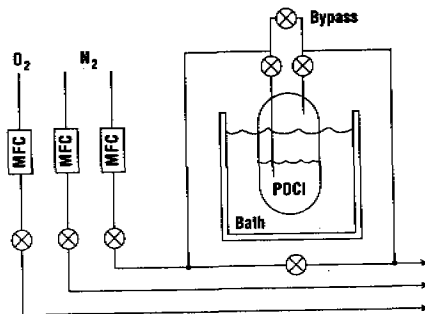
Figure 3.20 A typical bubbler arrangement for doping a silicon wafer using a \text{POCl}_3 source. The gas flow is set using mass flow controllers (MFC).
