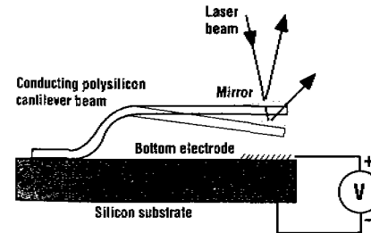
Figure 19.31 Illustration of electrostatic actuation of a cantilever beam micromirror. The insulating \text{SiO}_2 layer underneath the bottom electrode is not shown (after Muller [61], © 1998 IEEE).
