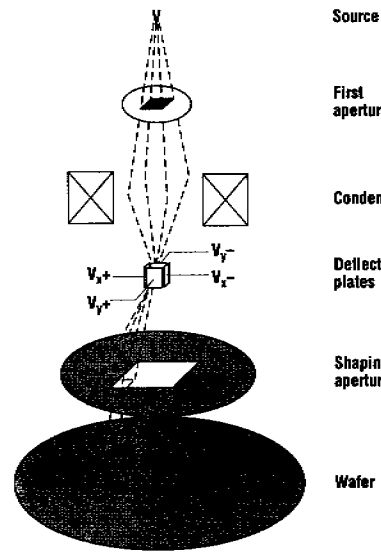
Figure 9.7 A variable shaped beam exposure system using mechanical beam stops for beam shaping. The broad beam exposes many pixels simultaneously, but dimensional control is not as reliable as standard EBL.
