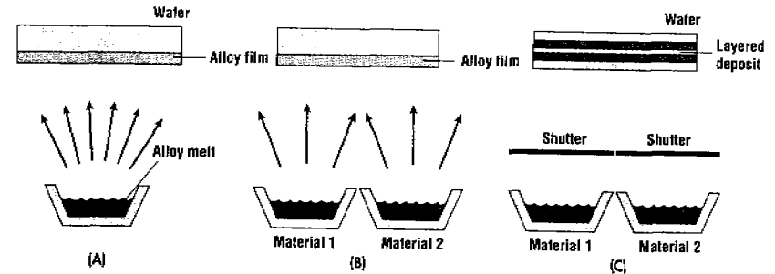
Figure 12.10 Methods for evaporating multicomponent films include (a) single source evaporation, (b) multisource simultaneous evaporation, and (c) multisource sequential evaporation.
