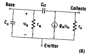
Figure 18.4 Small signal models of the bipolar transistor at (A) low frequency and (B) high frequency.
