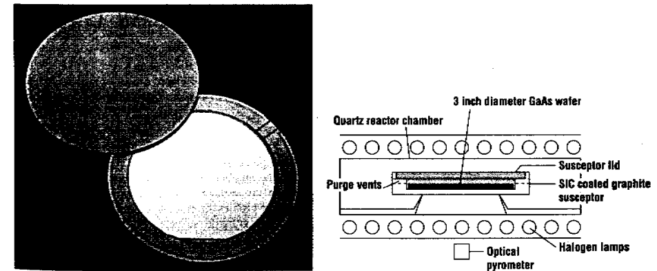
Figure 6.12 Photograph and schematic for capless arrangement for annealing GaAs (after Kazior et al., © 1991 IEEE).
