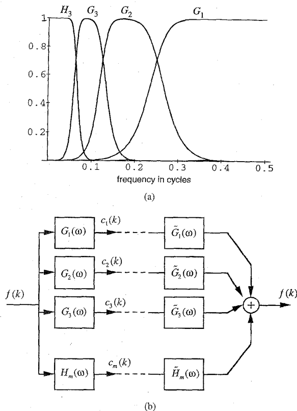
Fig. 1. Wavelets as a filterbank. (a) Multiband frequency response of the discrete filterbank associated with the cubic spline Battle-Lemarié wavelets. (b) Discrete perfect reconstruction filterbank without subsampling.
