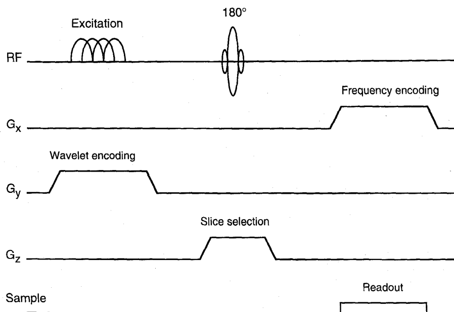
Fig. 5. Simplified representation of the pulse sequence used by Panich et al. for single section wavelet-encoded MRI. The sequence of events is as follows: 1) The sample is excited using a small flip angle wavelet-shaped RF pulse which is applied in conjunction with a linear gradient ( G_y ); this achieves a selective excitation in the y -direction. 2) The slice of interest is selected through the application of a spatially selective ( z -axis) sinc-shaped 180^\circ pulse. 3) Finally, the MR signal is measured with the x -gradient turned on; this achieves the frequency encoding in the x -direction.
